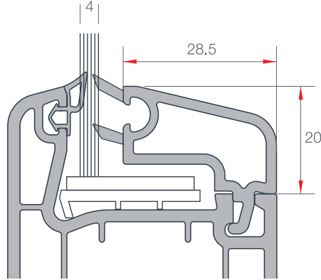
TEK CAM ÇİTASI SINGLE GLAZING BEAD EN 47
