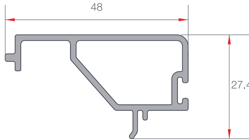
TEK RAYLI VSÜRME KASA EŞİK KAPAMA PROFİLİ THRESHOLD PROFILE FOR SINGLE RAILED SLIDING FRAME EN 69 0.340 gr/m
