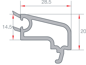
TEK CAM ÇITASI SLIDING SINGLE GLAZING BEAD EN 47 0.300 gr/m
