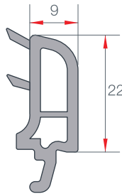
24 mm ÇİFT CAM ÇITASI SLIDING 24 mm DOUBLE GLAZING BEAD EN 109 0.225 gr/m
