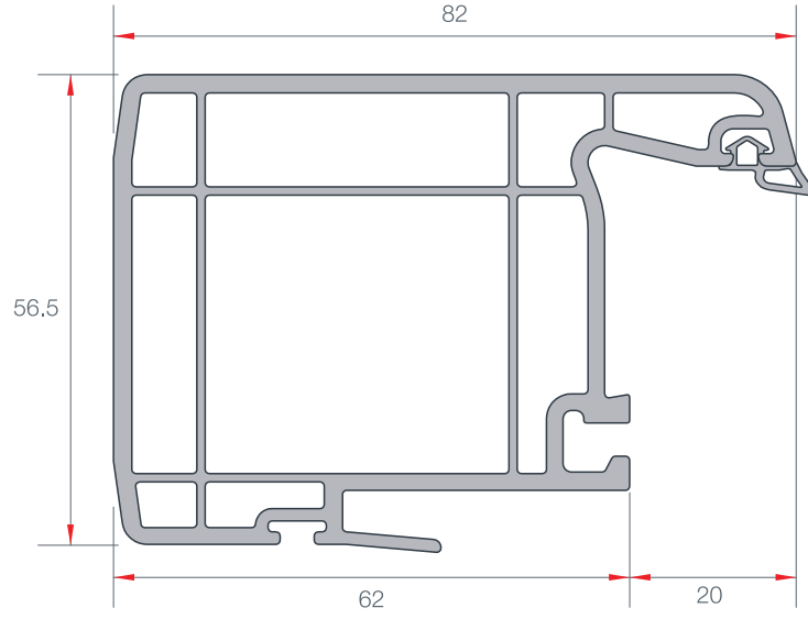
DİKEY ORTA KAYIT PROFİLİ SLIDING MULLION PROFILE EN 97 1.210 gr/m
