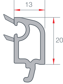
ÇİFT CAM ÇITASI SLIDING DOUBLE GLAZING BEAD EN 48 0.225 gr/m
