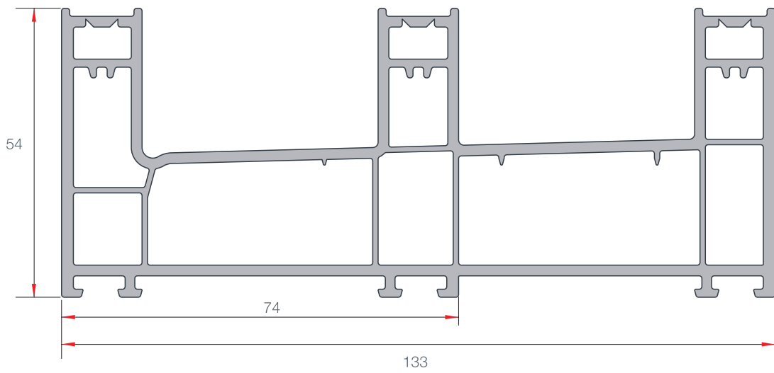
ÜÇ RAYLI KASA PROFİLİ TRIPLE RAILED SLIDING FRAME PROFILE EN 104 1.745 gr/m
