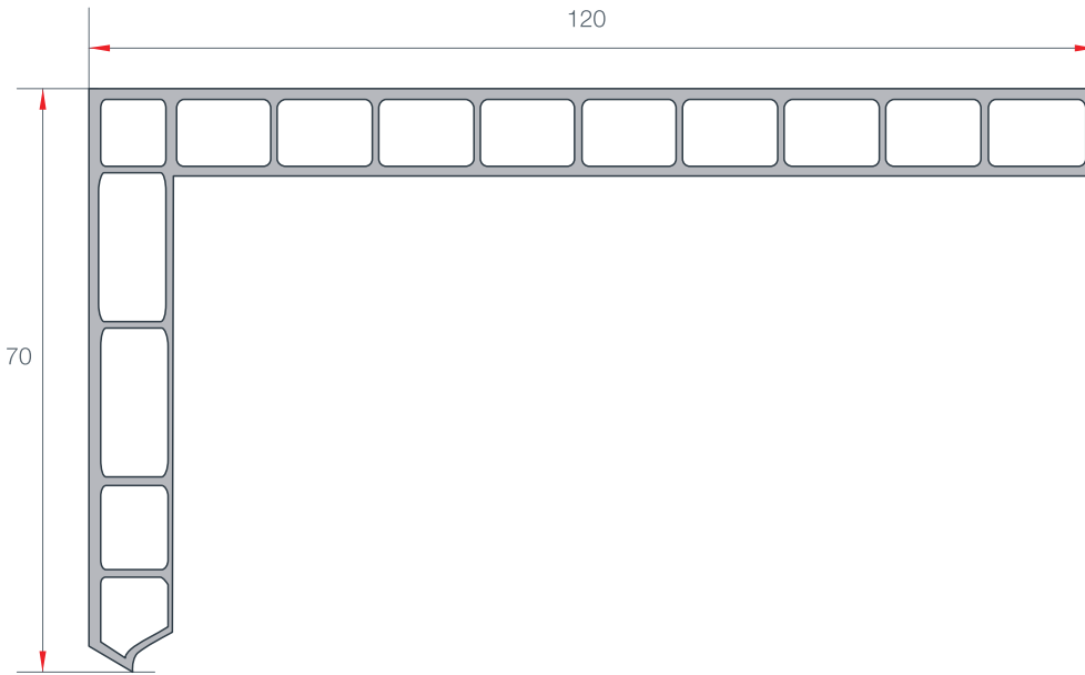
7 x 12 PERVAZ 7 X 12 COVER PROFILE EN 51
