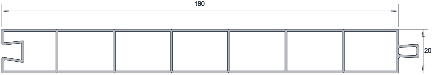
18 cm. LAMBRI 18.cm. PANEL PROFILE EN 59
