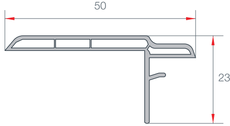
KLİPSLİ PERVAZ COVER PROFILE WITH CLIP EN 52
