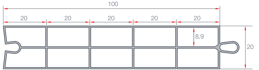
10 cm. LAMBRI 10.cm. PANEL PROFILE EN 60
