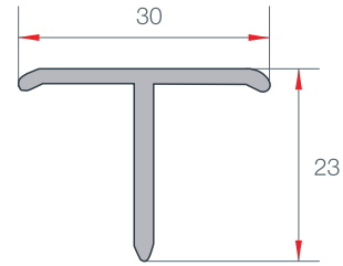
DAR "T" KAPAMA "T" PROFILE EN 63
