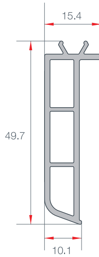
KLİPSLİ PERVAZ COVER PROFILE WITH CLIP EN 30 0.300 gr/m
